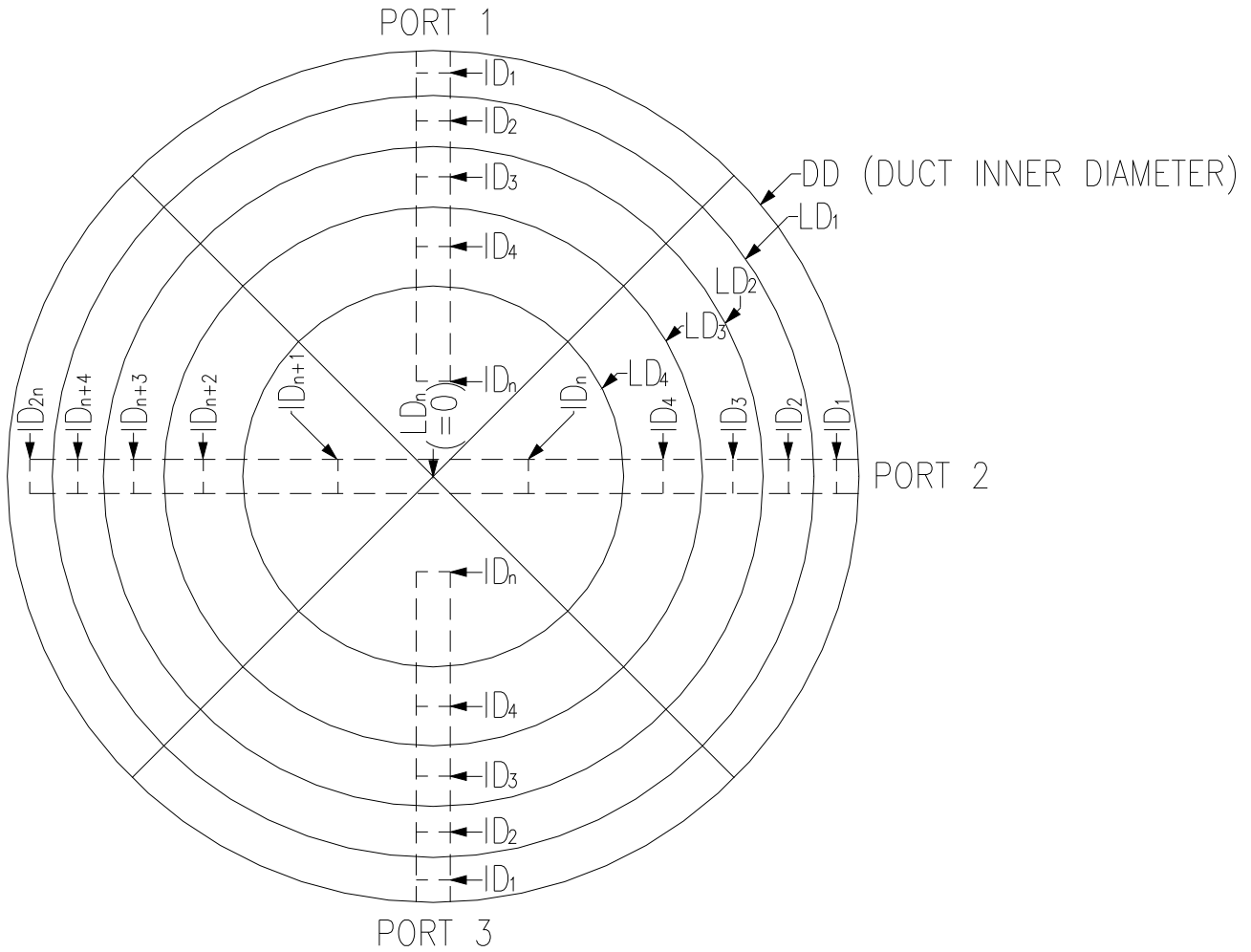
Cross-Section of Duct Perpendicular to Flow
